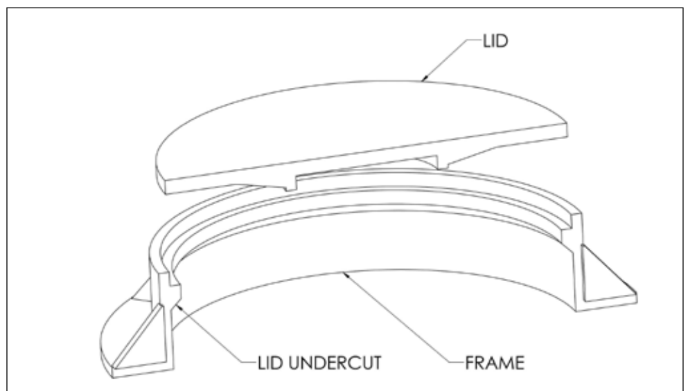
Figure 21. Lid Undercut
