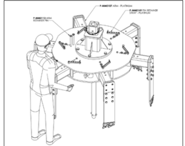
Figure 15. Setting Cutting Diameter
