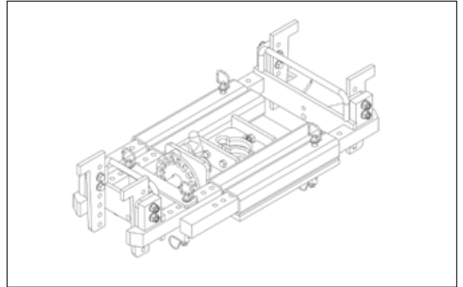
Figure 39. XL Speedplate
