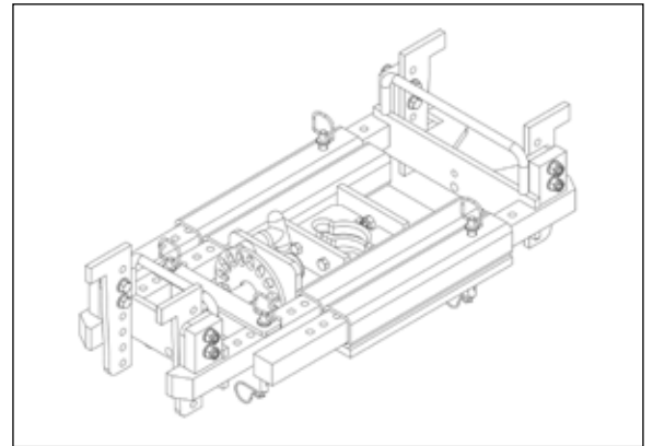
Figure 40. XL Speedplate
