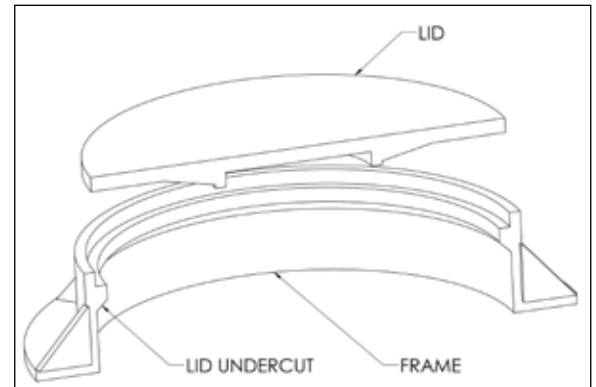
Figure 22. Lid Undercut
